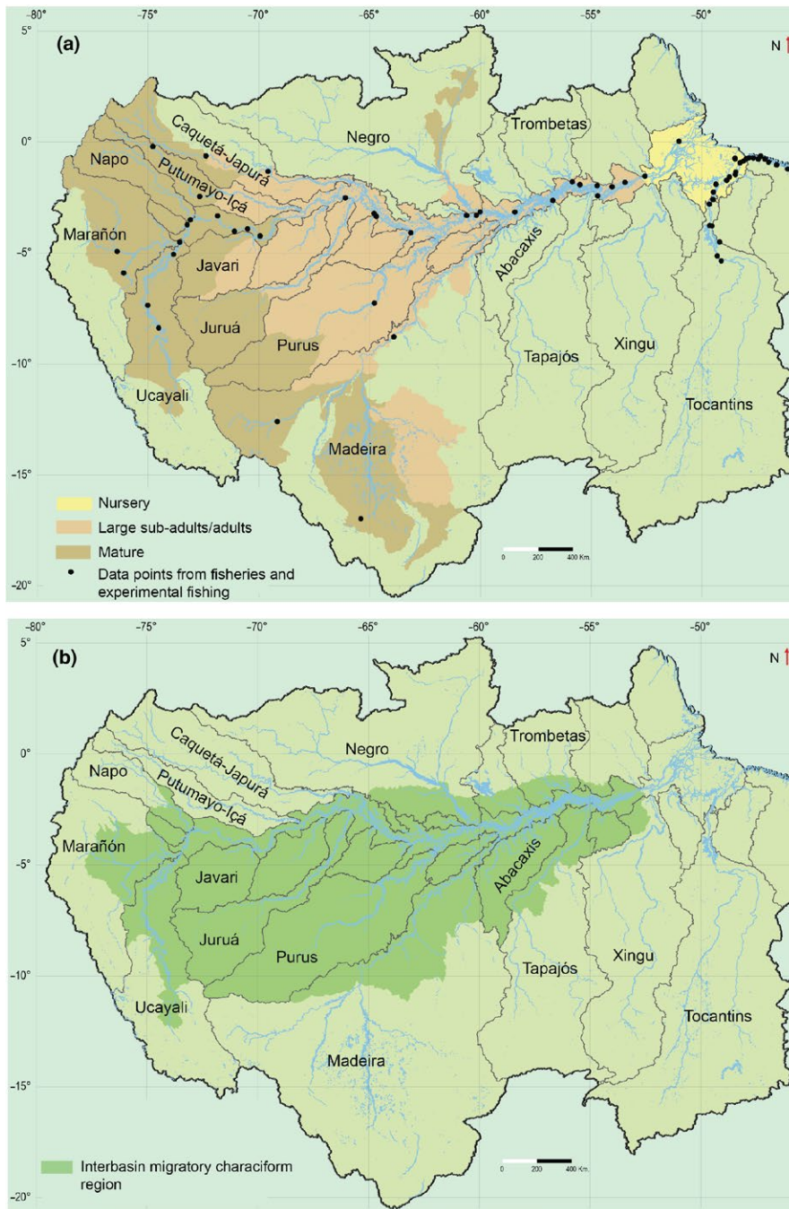
FIGURE 4 (a) The life-history region of dourada represents the largest management area of any interbasin migratory species. (b) The interbasin migratory characiform region that includes the main commercial fishing region and areas outside of it used for feeding
